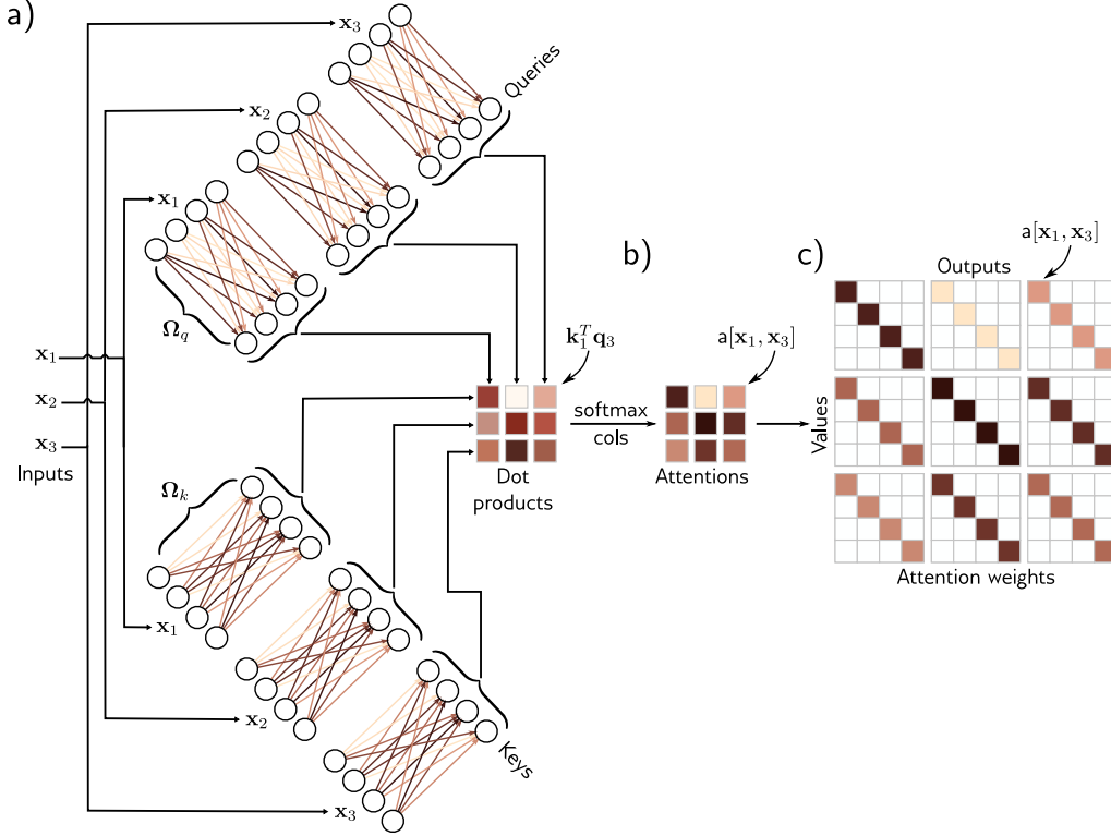
Figure 12.3 Computing attention weights. a) Query vectors q_n = \beta_q + \Omega_q x_n and key vectors k_n = \beta_k + \Omega_k x_n are computed for each input x_n . b) The dot products between each query and the three keys are passed through a softmax function to form non-negative attentions that sum to one. c) These route the value vectors (figure 12.1) via the sparse matrix from figure 12.2c.
